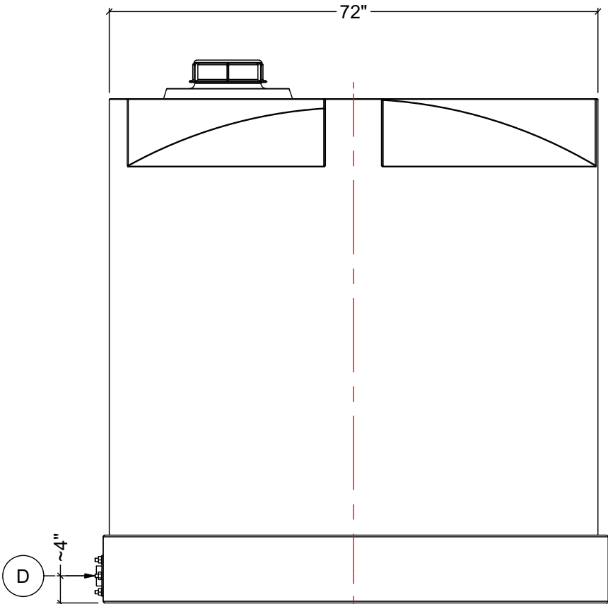
SIDE VIEW
