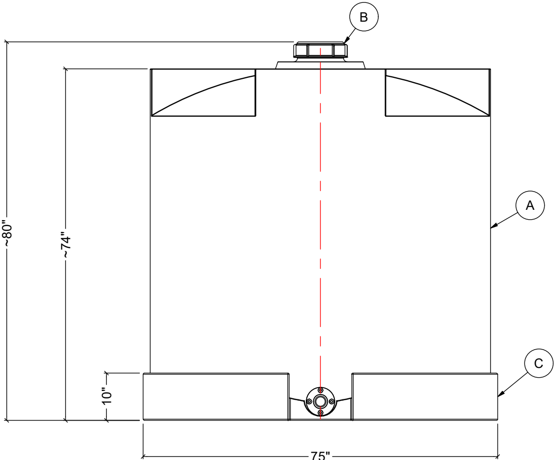
FRONT VIEW
