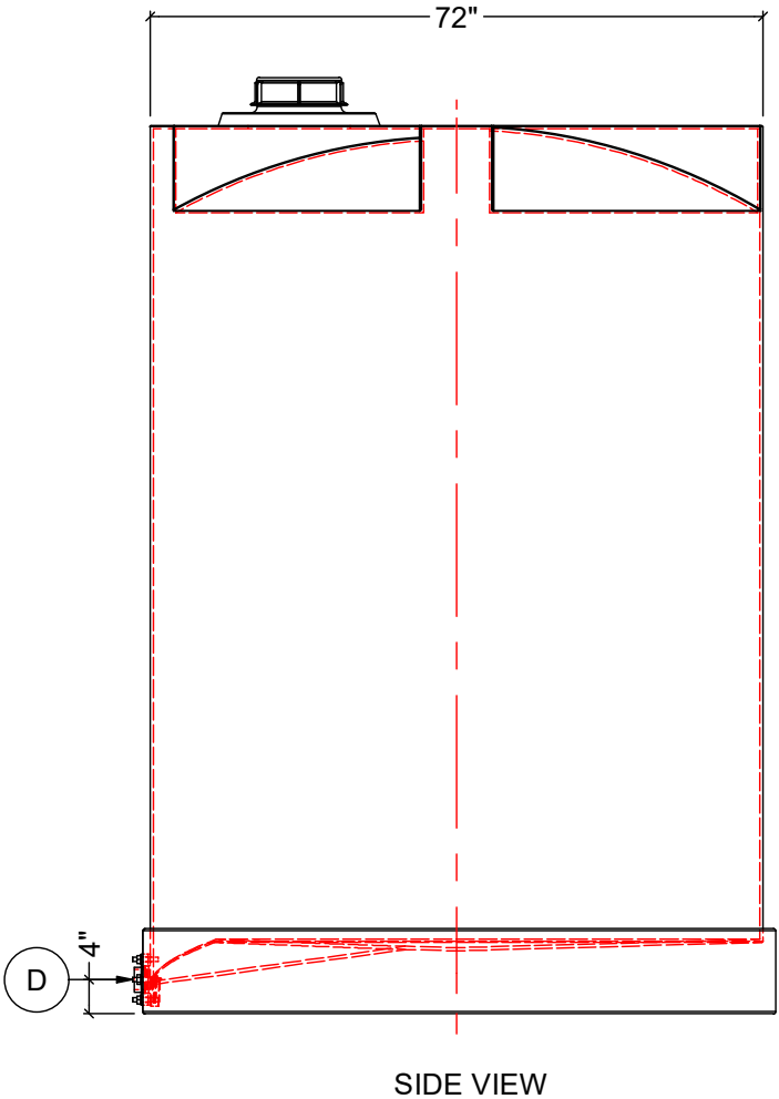
SIDE VIEW
