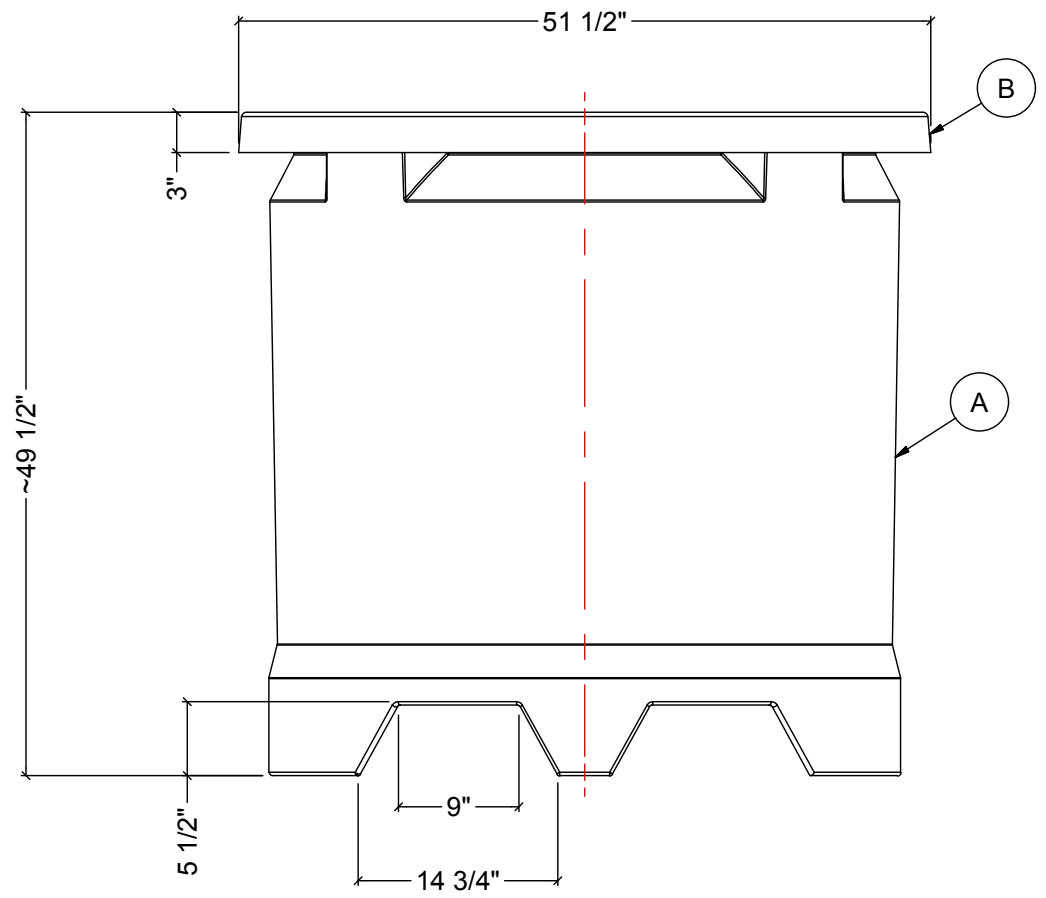
FRONT VIEW WITH COVER
