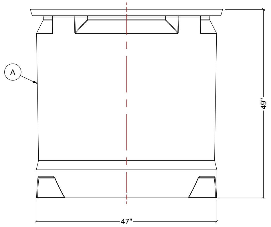
SIDE VIEW NO COVER
