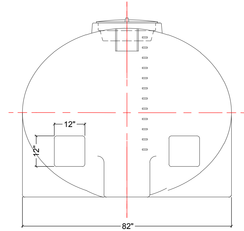
END VIEW
