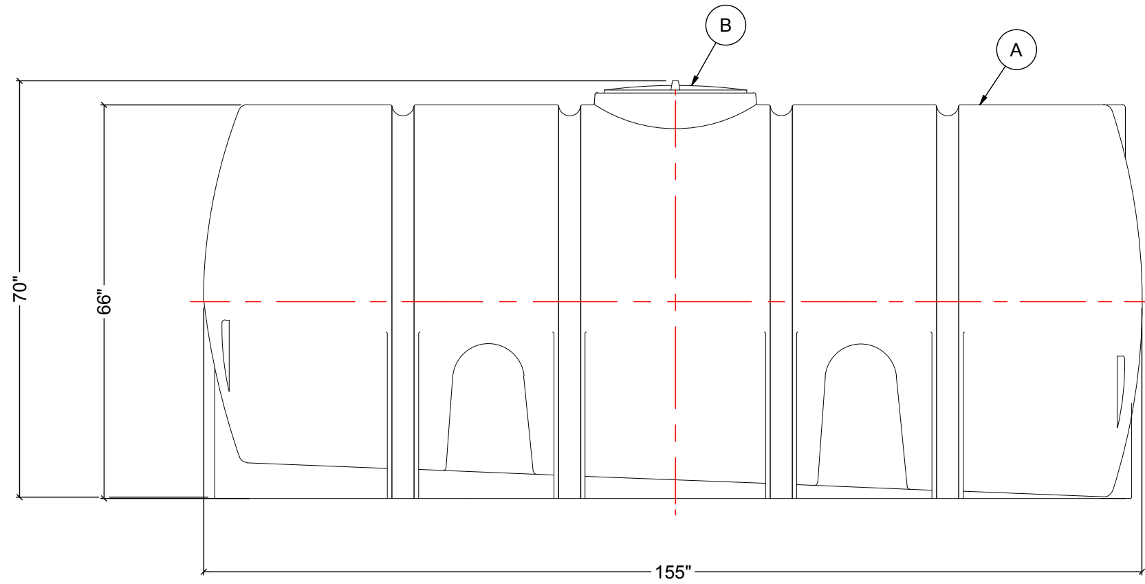
SIDE VIEW
