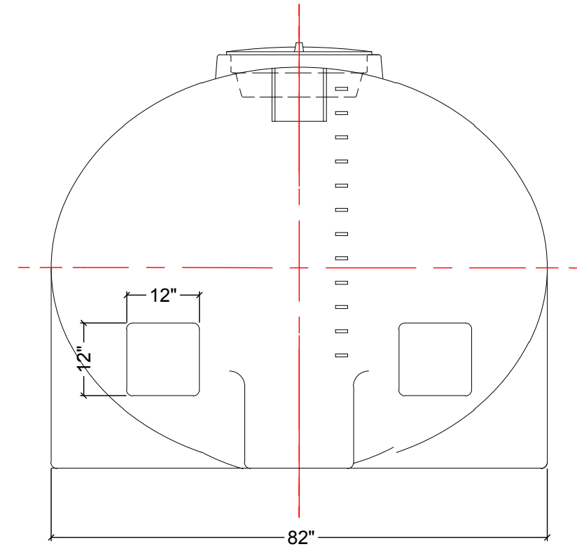
END VIEW
