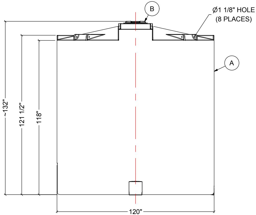
FRONT VIEW
