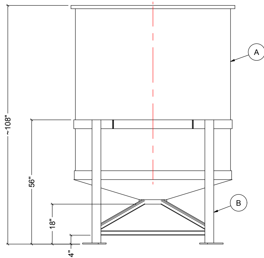
FRONT VIEW
