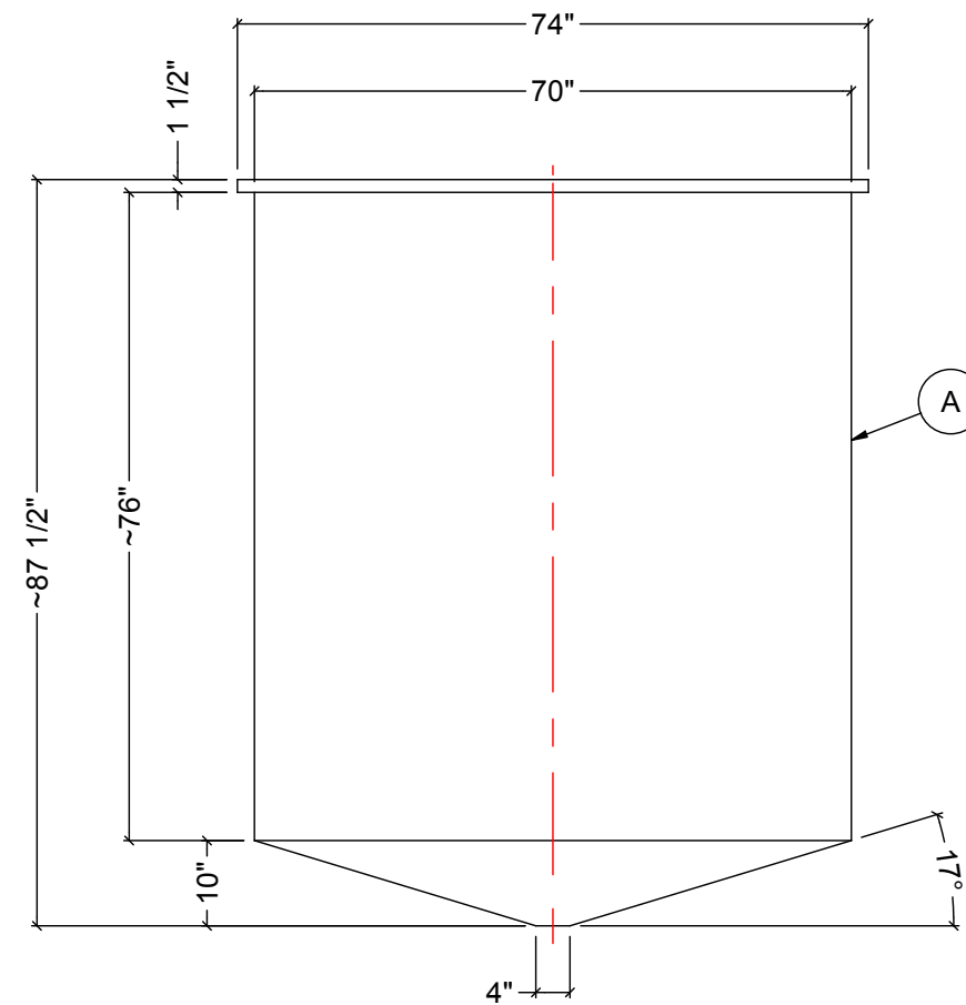
SIDE VIEW - NO STAND
