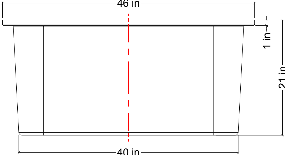
FRONT VIEW
