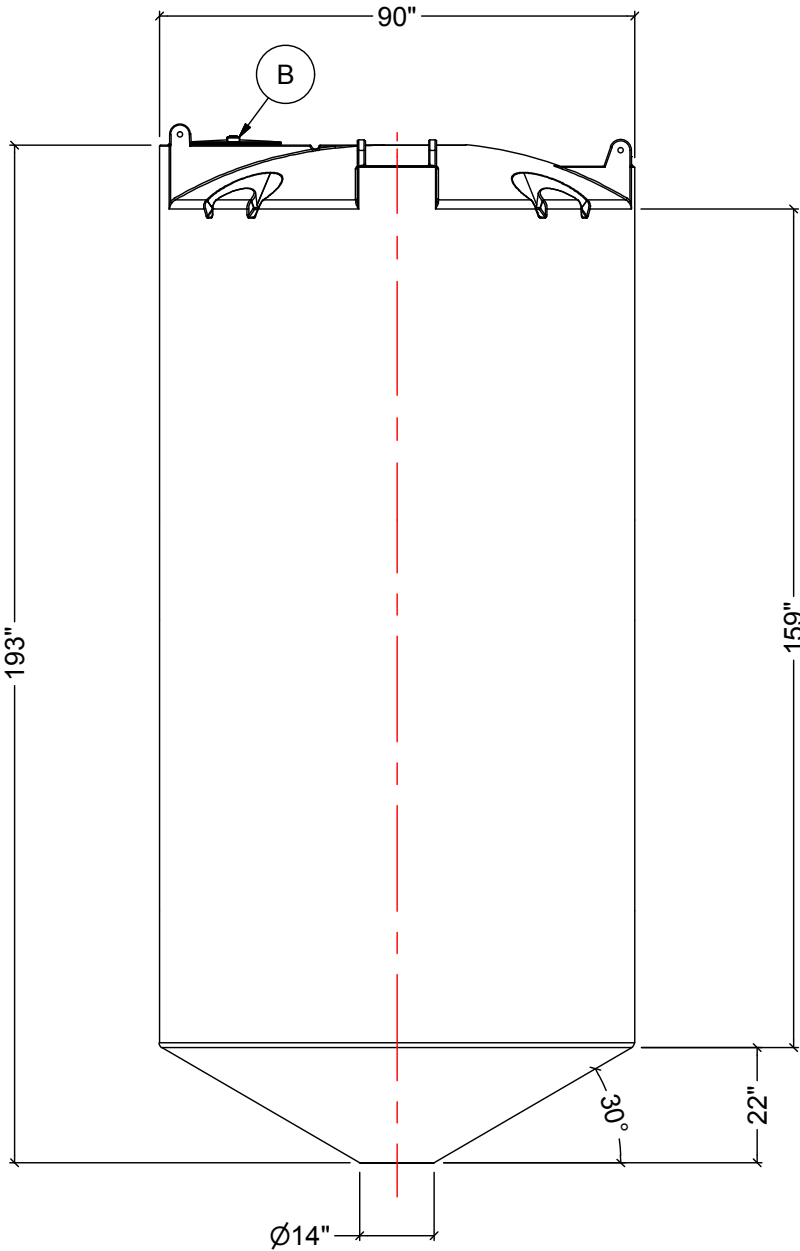
SIDE VIEW
