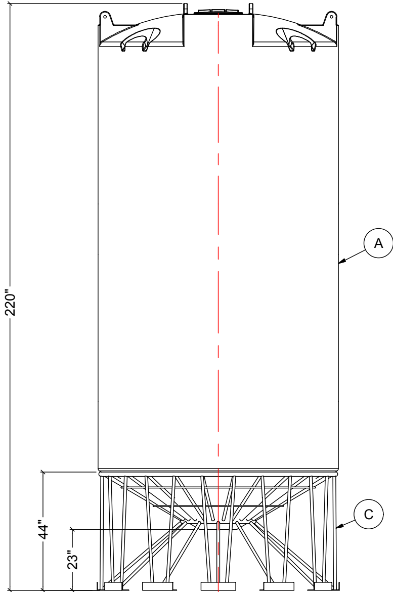
FRONT VIEW
