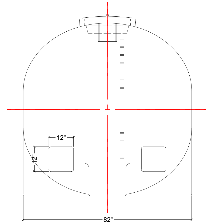
END VIEW
