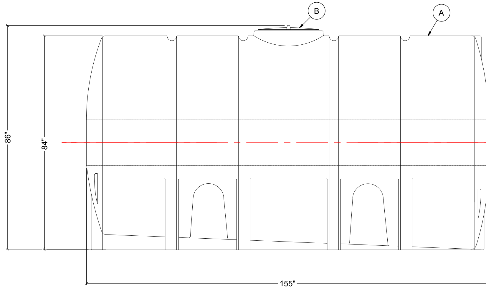
SIDE VIEW
