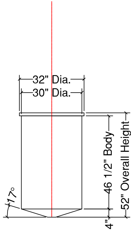
FRONT VIEW
