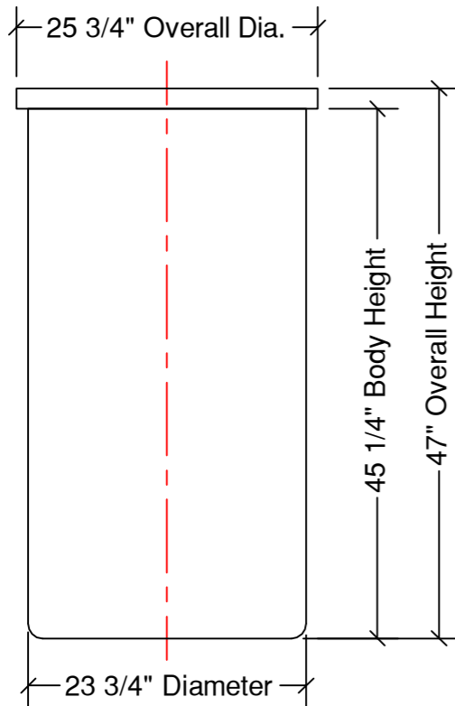
FRONT VIEW
