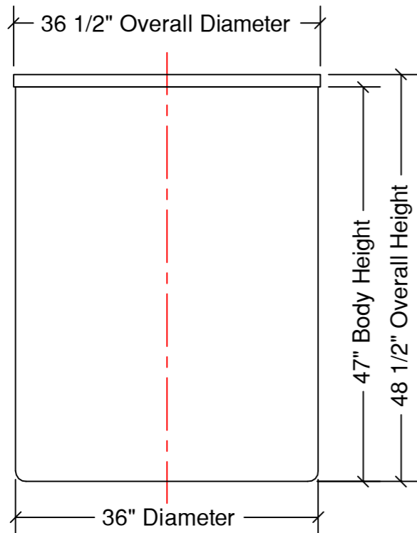
FRONT VIEW
